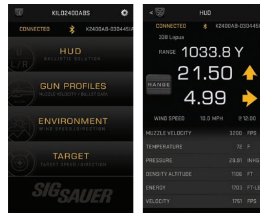
KILO2400ABS syncs with a smart phone via the Applied Ballistic's Ballistic Solver app. Calculating long-range rifle trajectories for the perfect shot. (Smart phone app display shown.)
